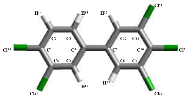
Figure 1. The optimized geometry of 33'44'5-pentachloro biphenyl (PCBP) with the atom numbering.
