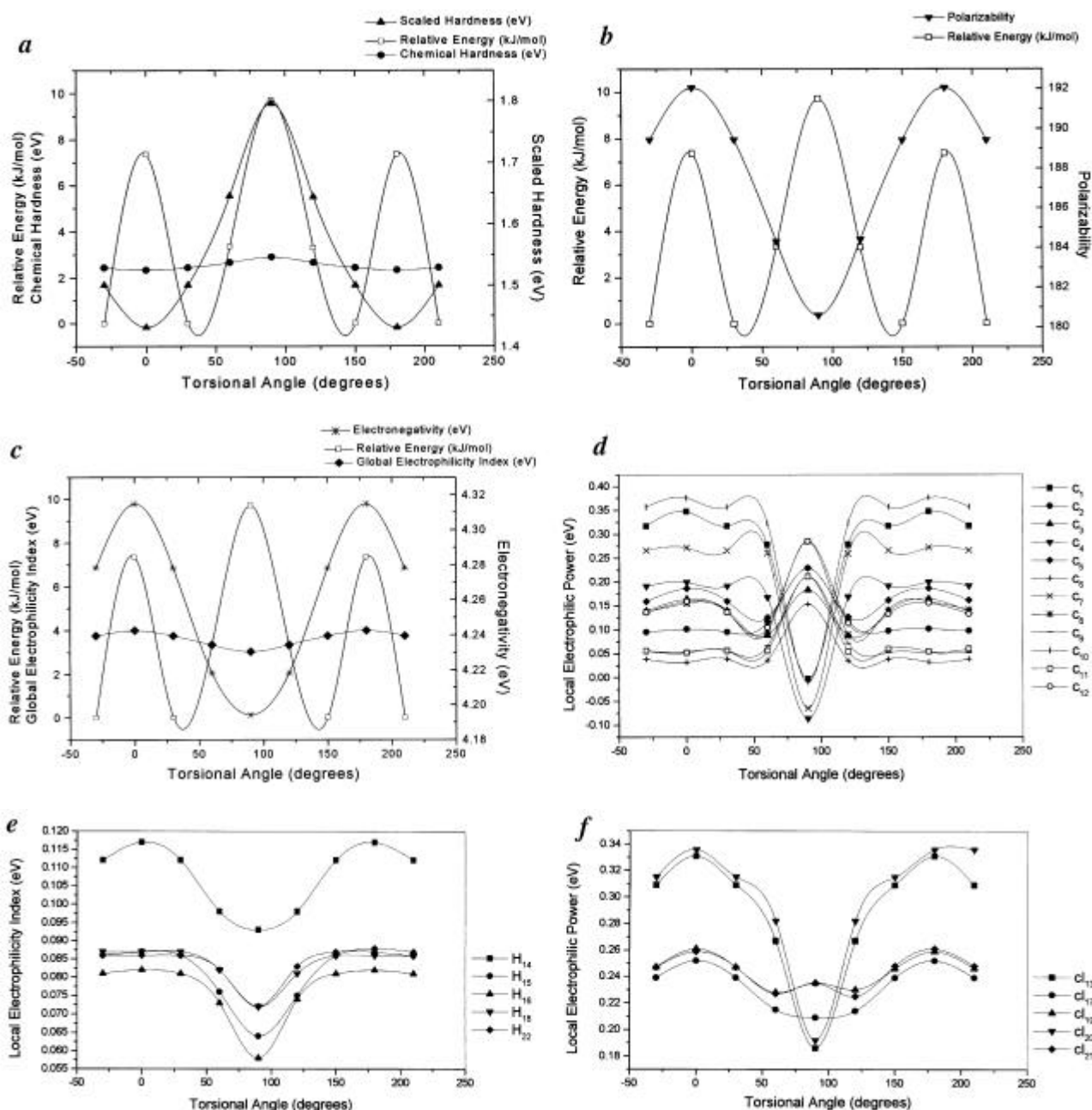
Figure 2. a, The variation of relative energy (kJ/mol), chemical hardness (eV) and scaled hardness (eV) with the torsional angle (degrees) for 33'44'5-PCBP. b, The variation of polarizability and relative energy (kJ/mol) with the torsional angle (degrees) for 33'44'5-PCBP. c, The variation of relative energy (kJ/mol), electronegativity (eV) and global electrophilicity index (eV) with the torsional angle (degrees) for 33'44'5-PCBP. d, The variation of local electrophilic power (eV) with the torsional angle (degrees) for C atoms in 33'44'5-PCBP. e, The variation of local electrophilic power (eV) with the torsional angle (degrees) for H atoms in 33'44'5-PCBP. f, The variation of local electrophilic power (eV) with the torsional angle (degrees) for Cl atoms in 33'44'5-PCBP.
